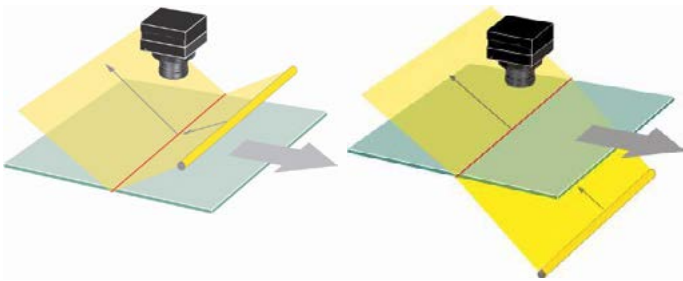
Two sample illumination setups: Dark field illumination in reflection (left) and in transmission (right)
