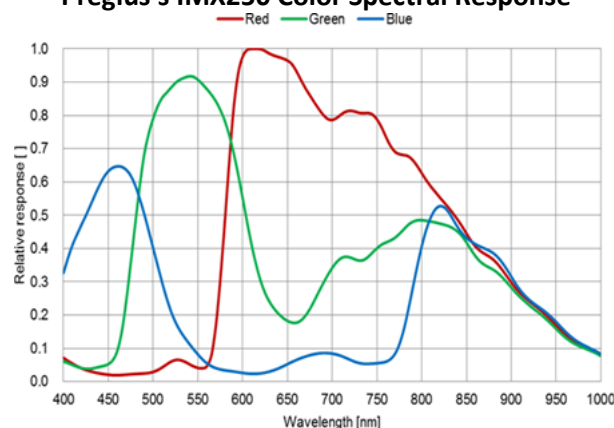
Pregius's IMX250 Color Spectral Response
