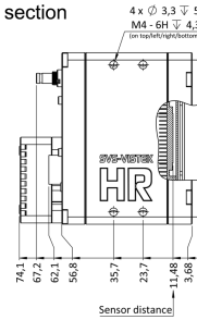
cross section
