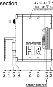
cross section
